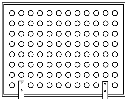
Special perforation D 50 mm
