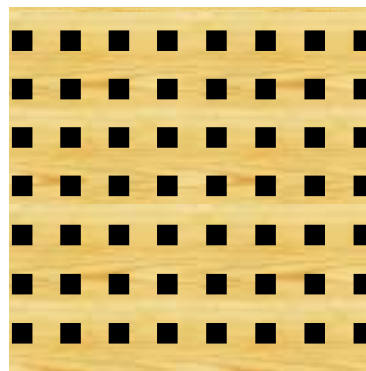
Hole size 12x12 mm, sharing cc 32,5 mm Hole area 14 %.
