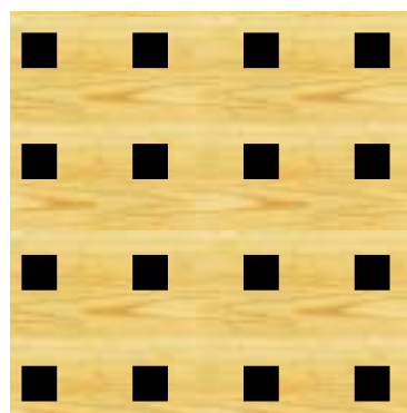
Hole size 20x20 mm, sharing cc 66 mm Hole area 9 %.
